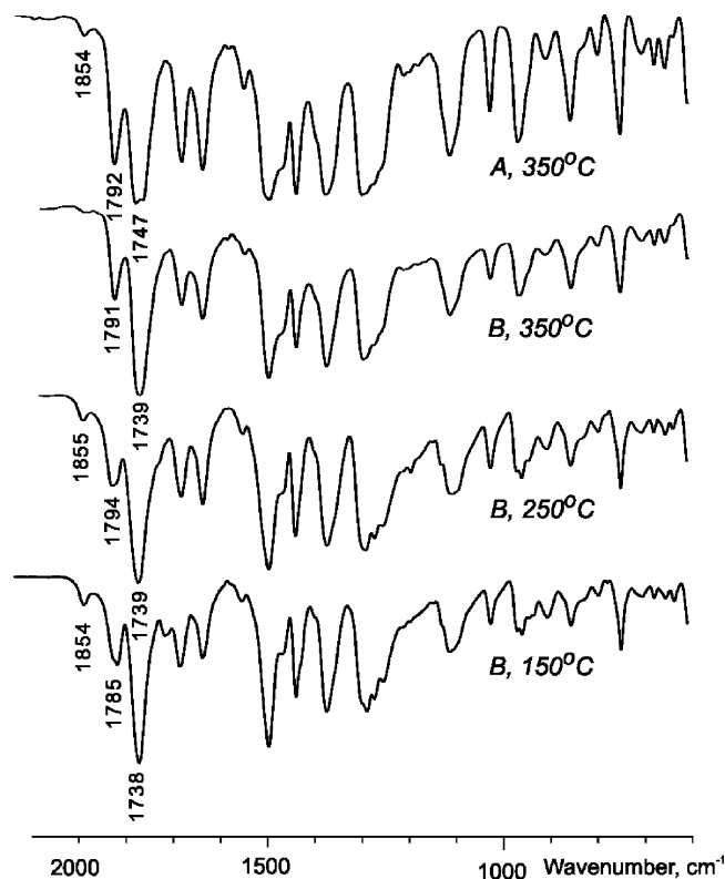
Fig. 1. FTIR spectra of PI-1 (2,7-DAHFN/ODPA) during polycondensation by methods A and B at different T c (in KBr). The absorption at ~1790 and 1740 cm -1 is assigned to the stretching vibrations of imide group carbonyl, 1855 cm -1 —anhydride group carbonyl.
